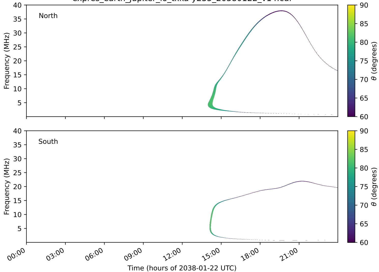
expres_earth_jupiter_io_txka-y235_20380122_v14.cdf
