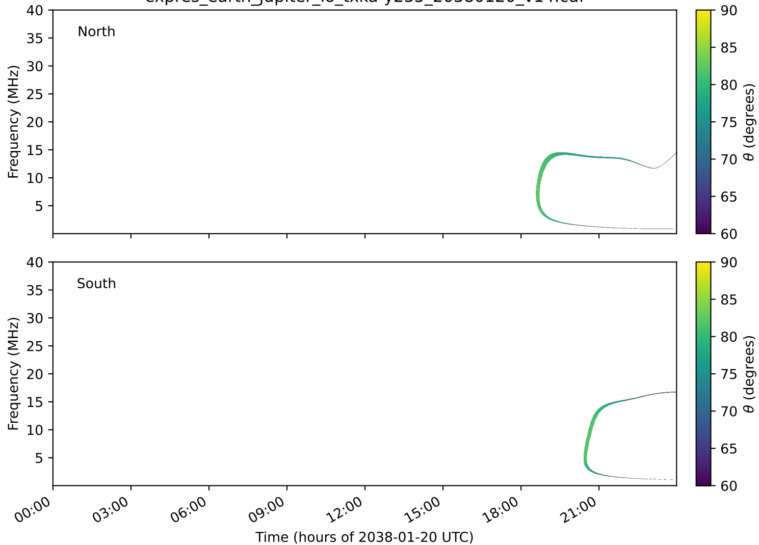
expres_earth_jupiter_io_txka-y235_20380120_v14.cdf
