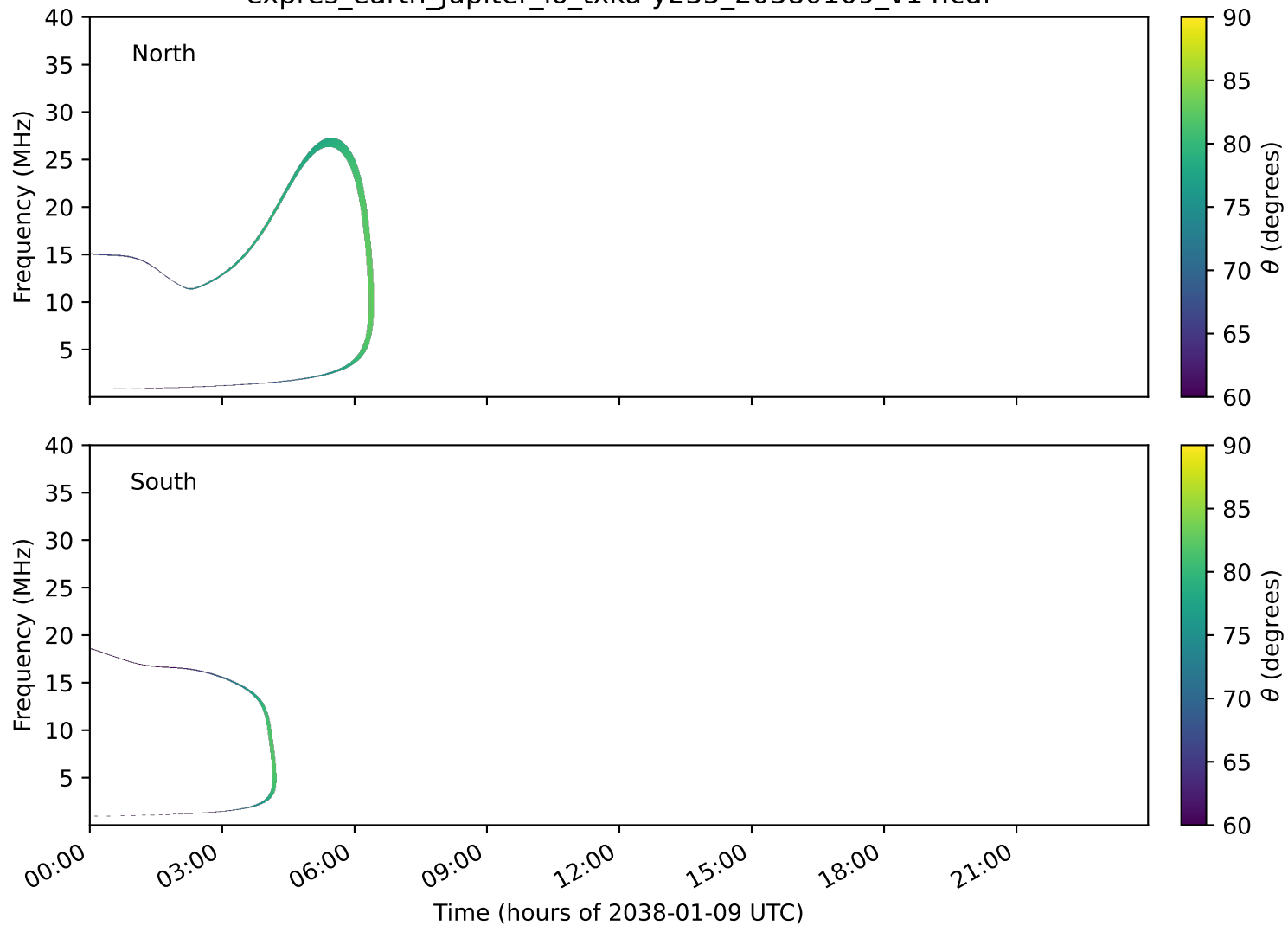
expres_earth_jupiter_io_txka-y235_20380109_v14.cdf
