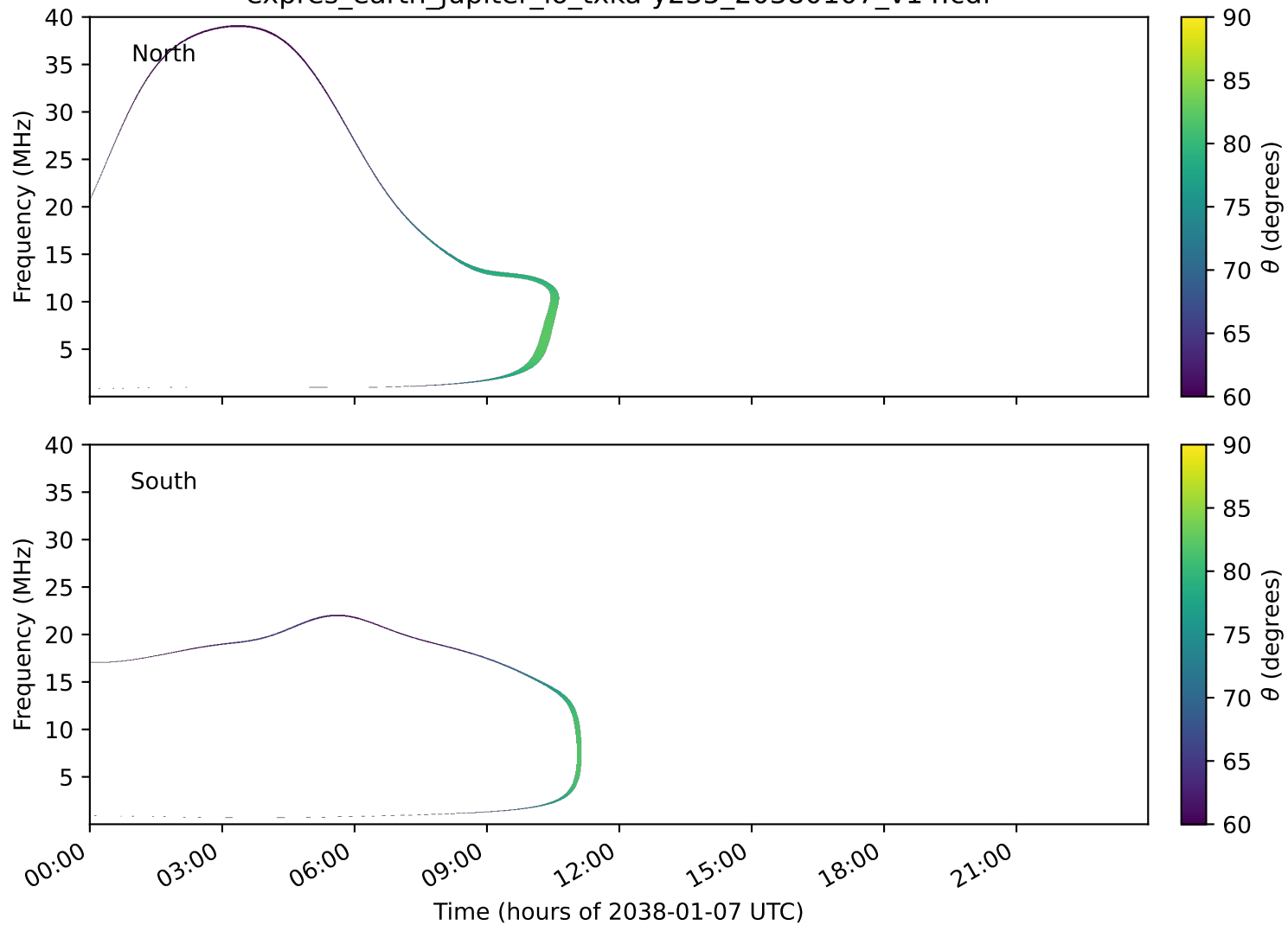
expres_earth_jupiter_io_txka-y235_20380107_v14.cdf
