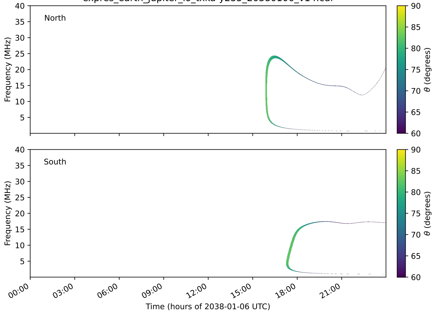
expres_earth_jupiter_io_txka-y235_20380106_v14.cdf
