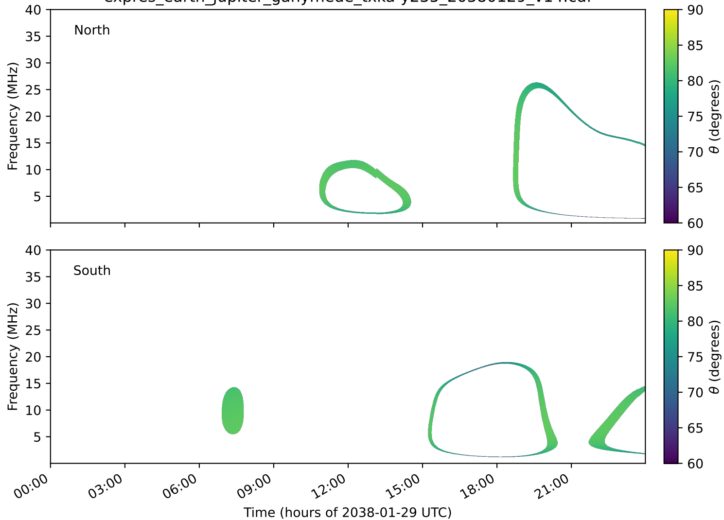
expres_earth_jupiter_ganymede_txka-y235_20380129_v14.cdf
