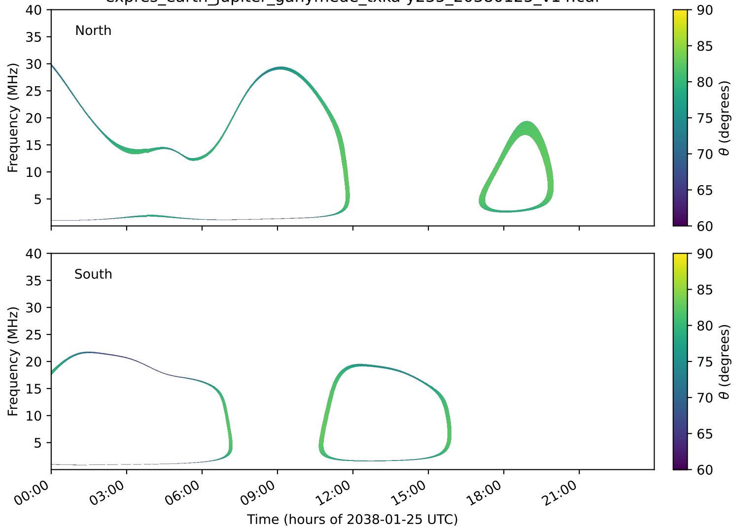
expres_earth_jupiter_ganymede_txka-y235_20380125_v14.cdf
