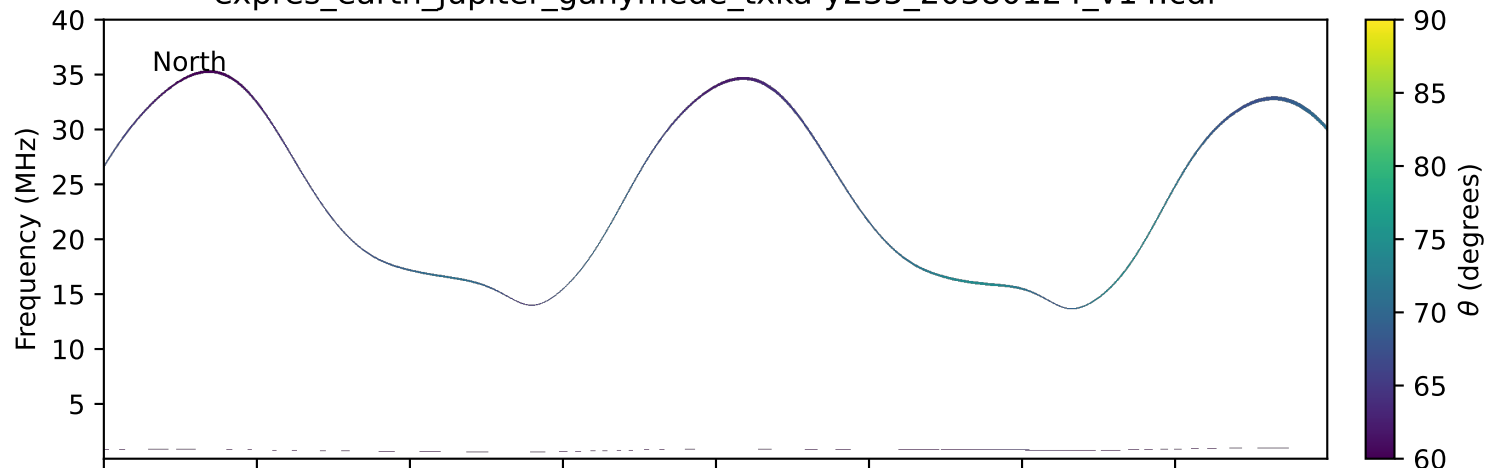
expres_earth_jupiter_ganymede_txka-y235_20380124_v14.cdf
