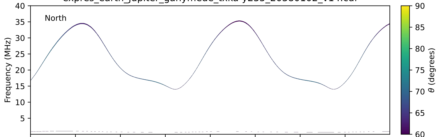
expres_earth_jupiter_ganymede_txka-y235_20380102_v14.cdf
