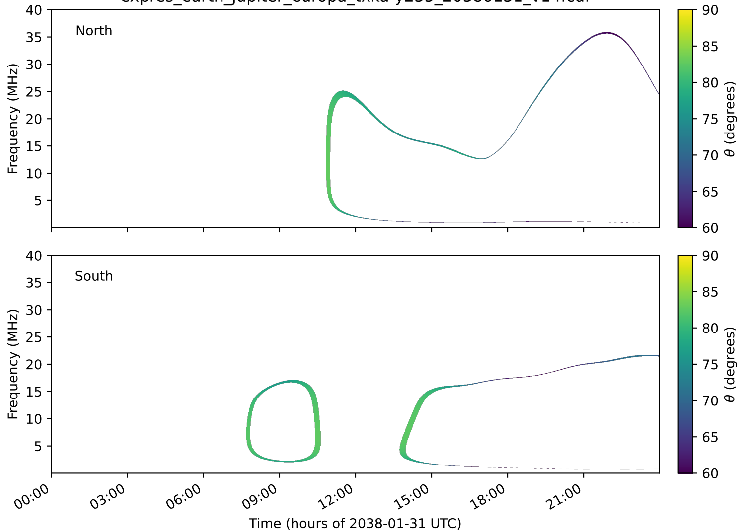
expres_earth_jupiter_europa_txka-y235_20380131_v14.cdf
