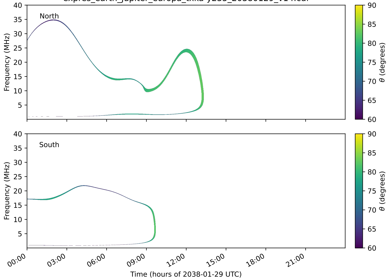
expres_earth_jupiter_europa_txka-y235_20380129_v14.cdf
