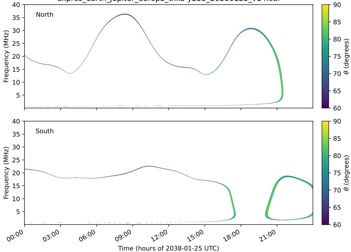
expres_earth_jupiter_europa_txka-y235_20380125_v14.cdf
