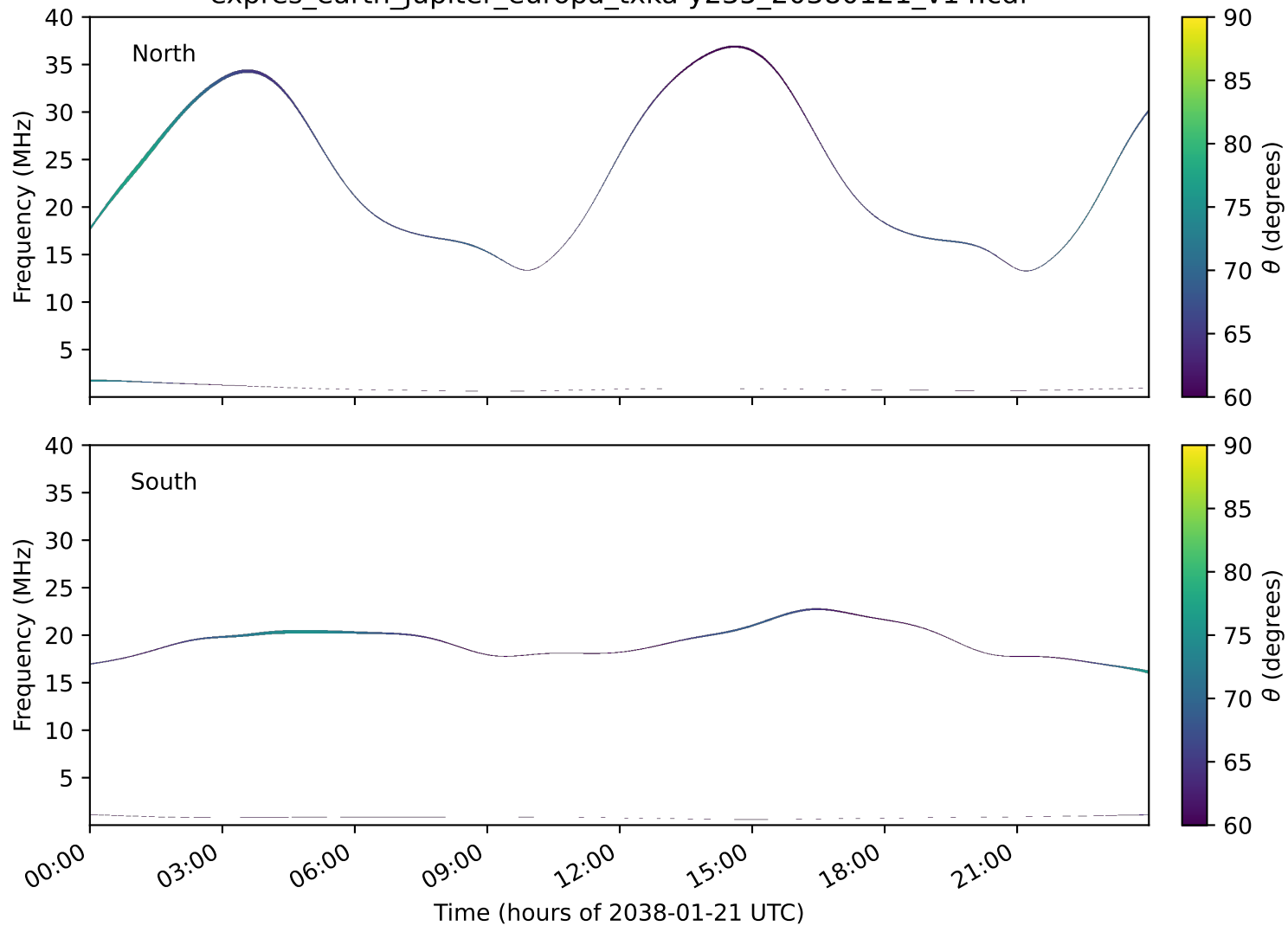
expres_earth_jupiter_europa_txka-y235_20380121_v14.cdf
