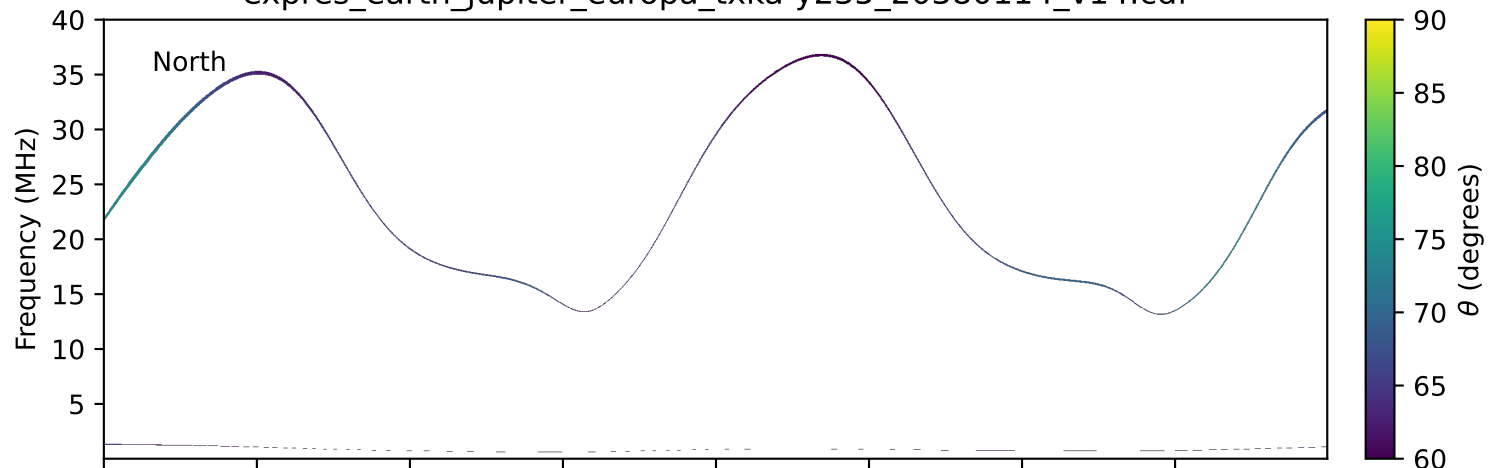
expres_earth_jupiter_europa_txka-y235_20380114_v14.cdf
