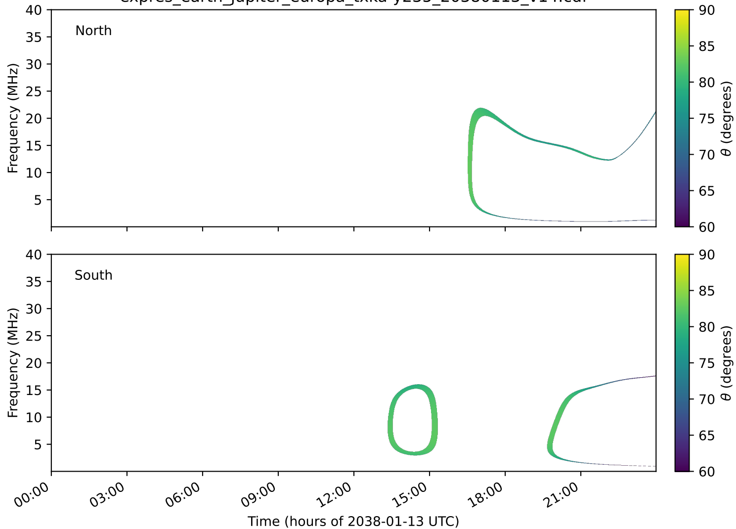
expres_earth_jupiter_europa_txka-y235_20380113_v14.cdf
