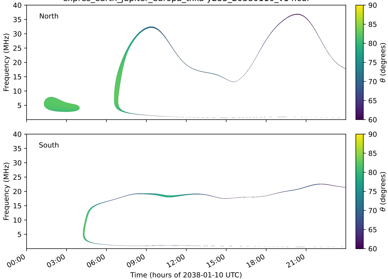
expres_earth_jupiter_europa_txka-y235_20380110_v14.cdf
