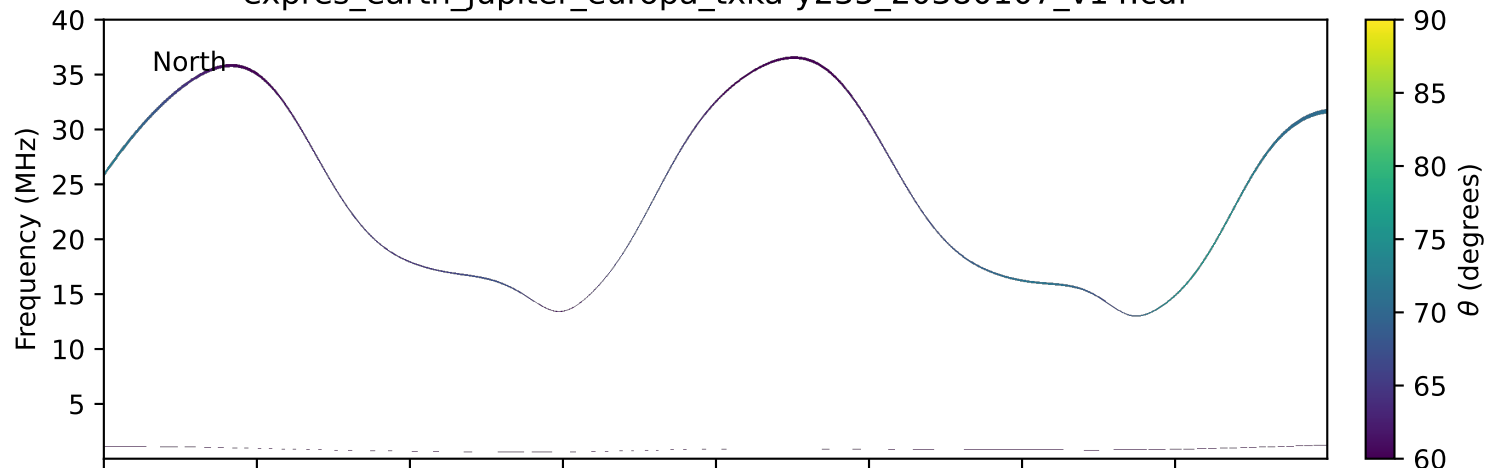
expres_earth_jupiter_europa_txka-y235_20380107_v14.cdf
