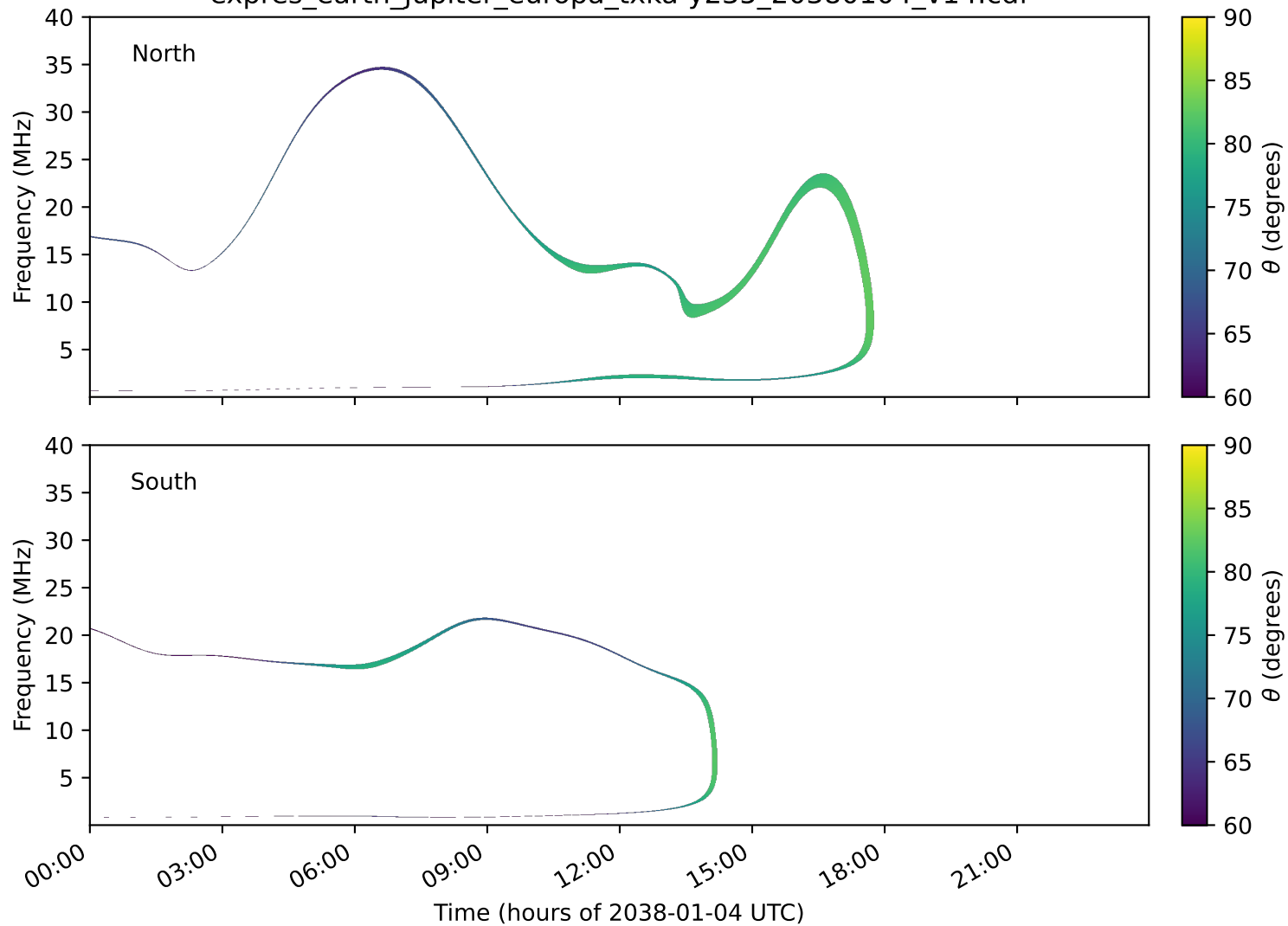
expres_earth_jupiter_europa_txka-y235_20380104_v14.cdf
