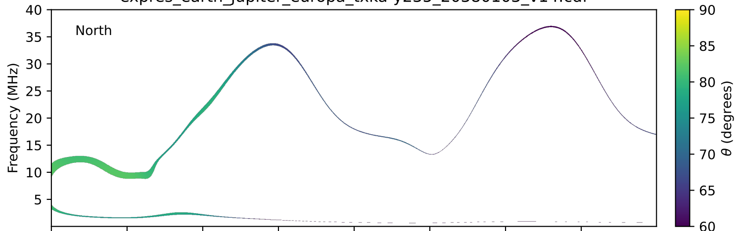
expres_earth_jupiter_europa_txka-y235_20380103_v14.cdf
