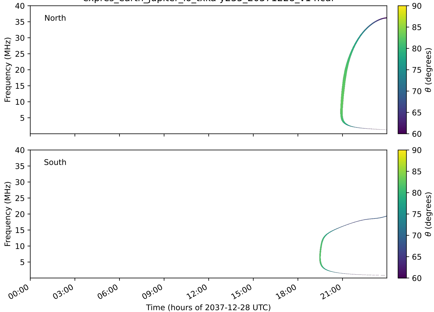
expres_earth_jupiter_io_txka-y235_20371228_v14.cdf
