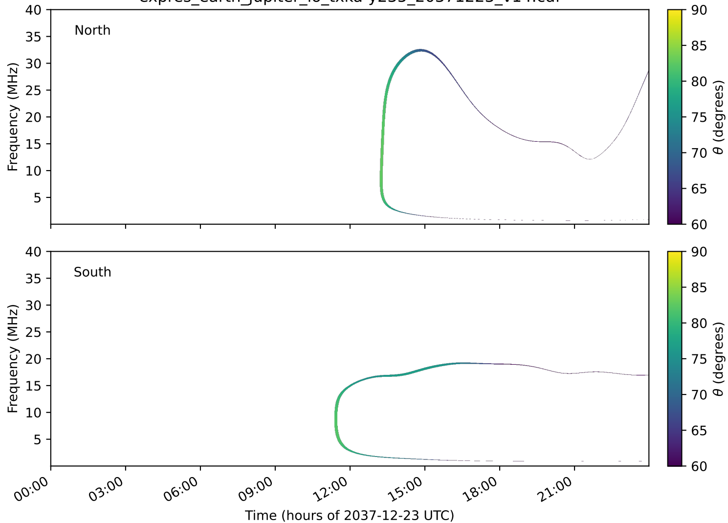
expres_earth_jupiter_io_txka-y235_20371223_v14.cdf
