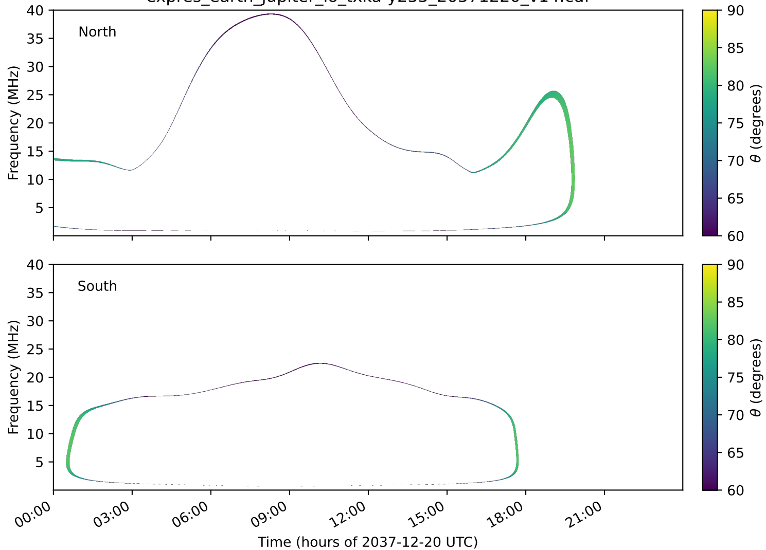
expres_earth_jupiter_io_txka-y235_20371220_v14.cdf
