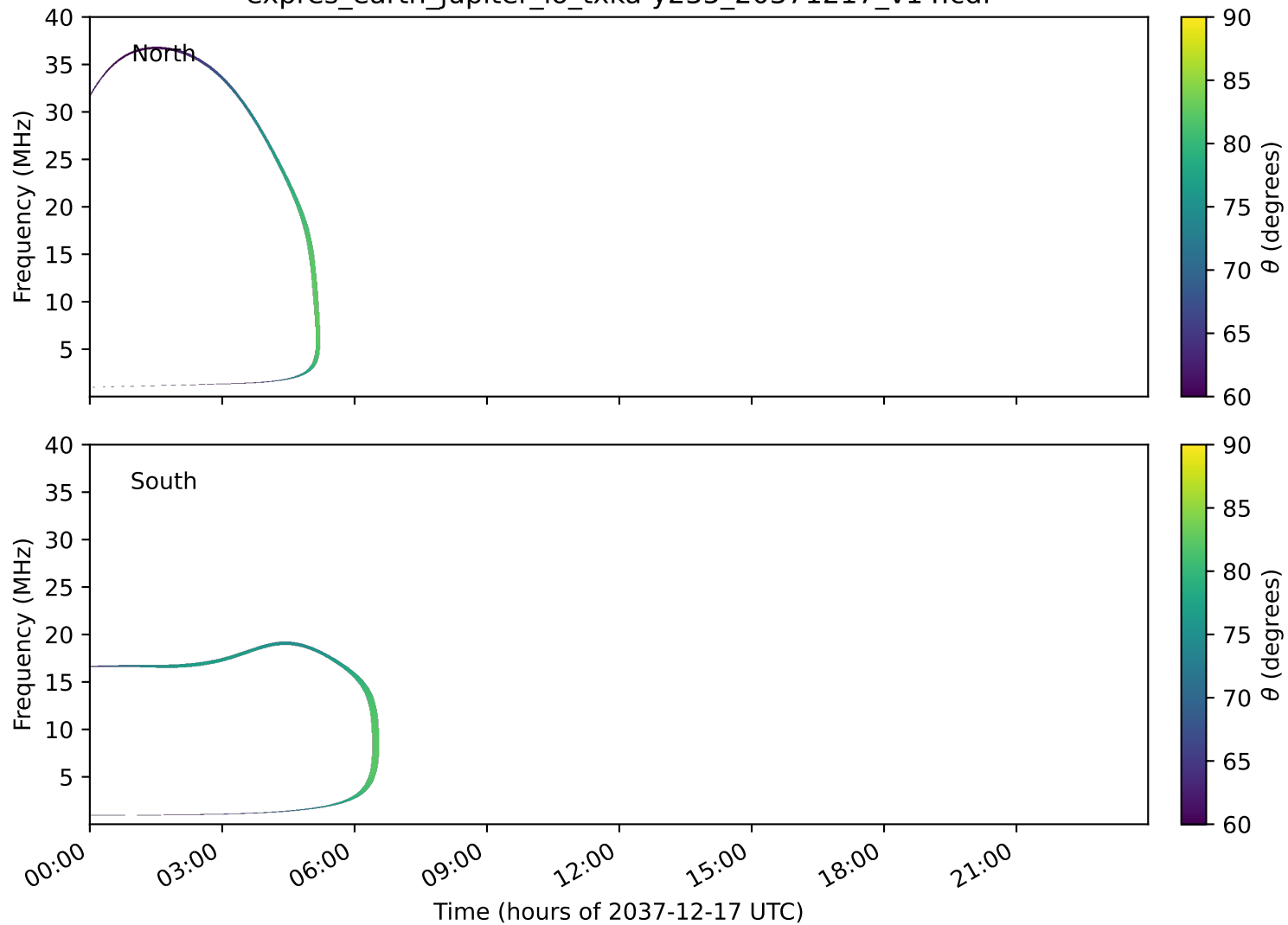
expres_earth_jupiter_io_txka-y235_20371217_v14.cdf
