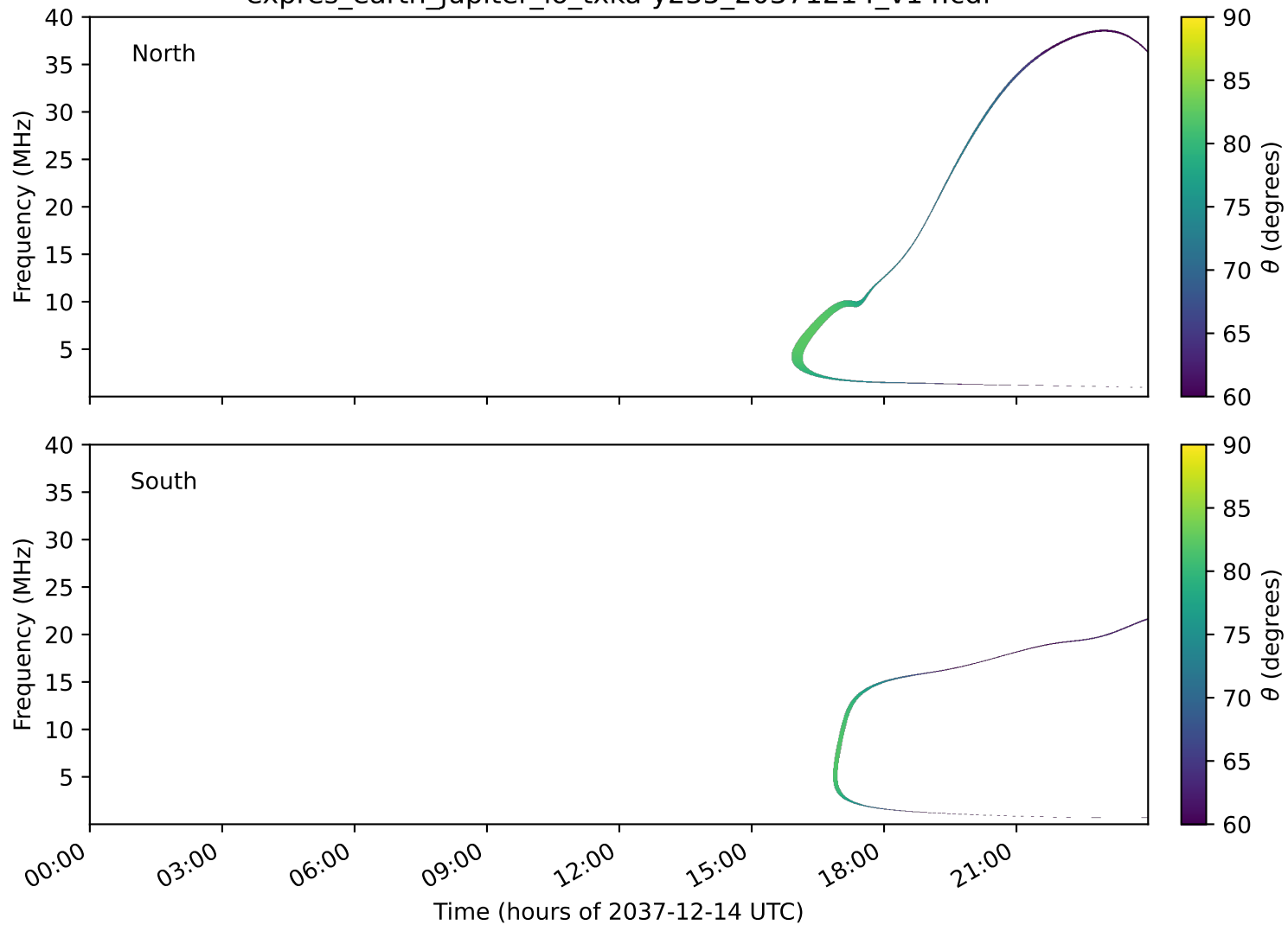
expres_earth_jupiter_io_txka-y235_20371214_v14.cdf
