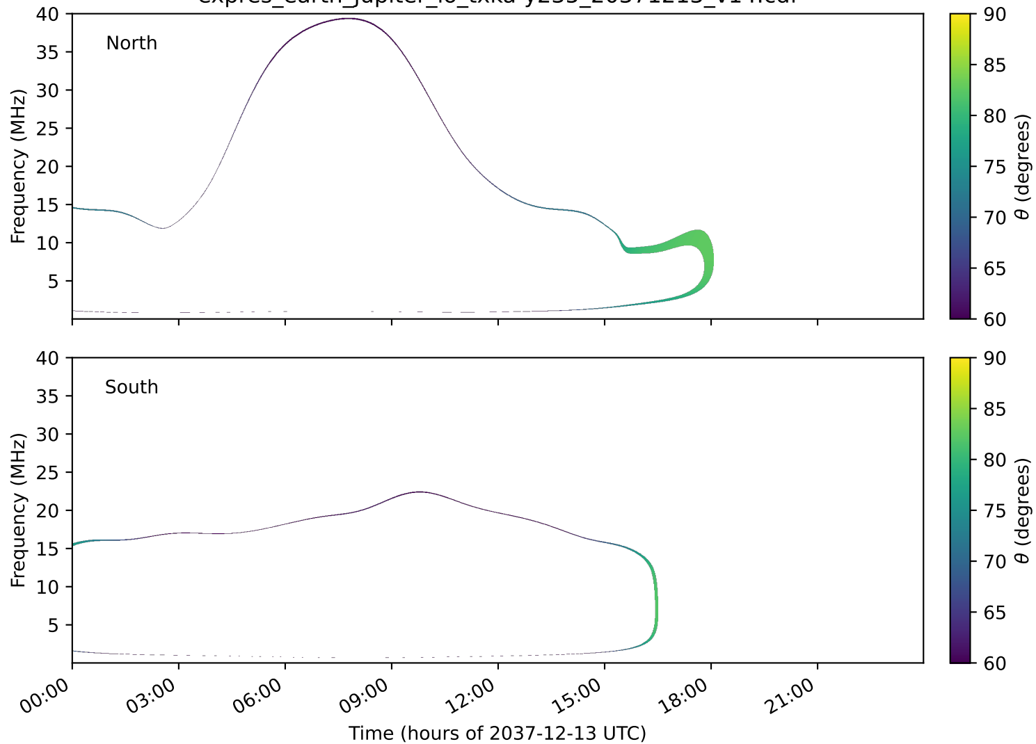
expres_earth_jupiter_io_txka-y235_20371213_v14.cdf
