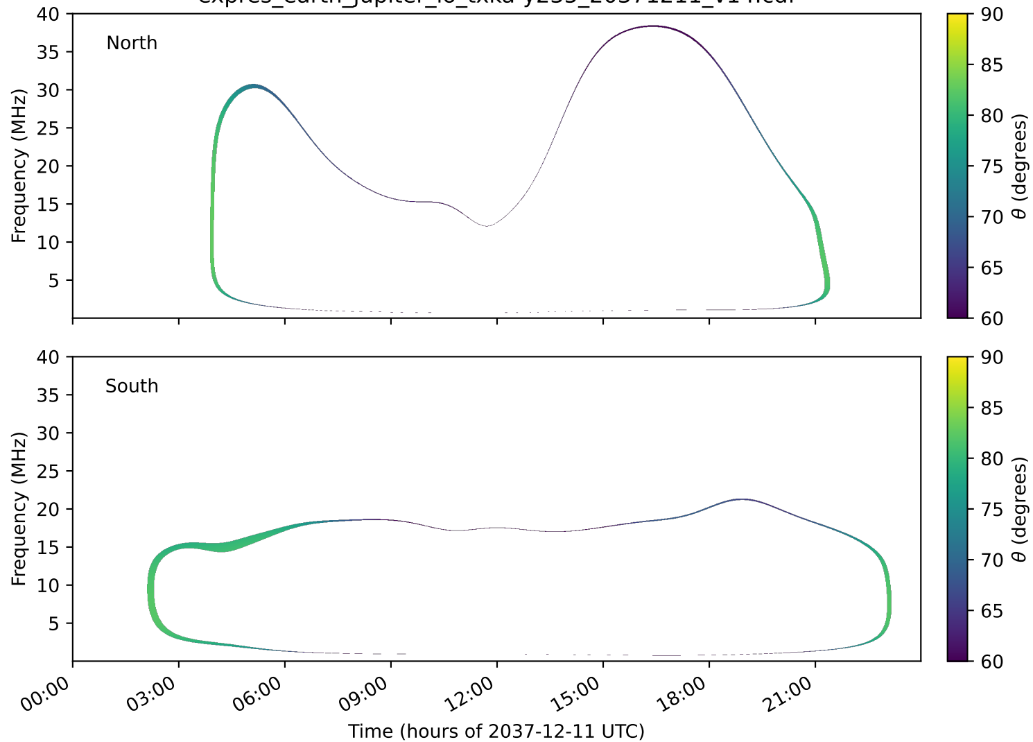
expres_earth_jupiter_io_txka-y235_20371211_v14.cdf
