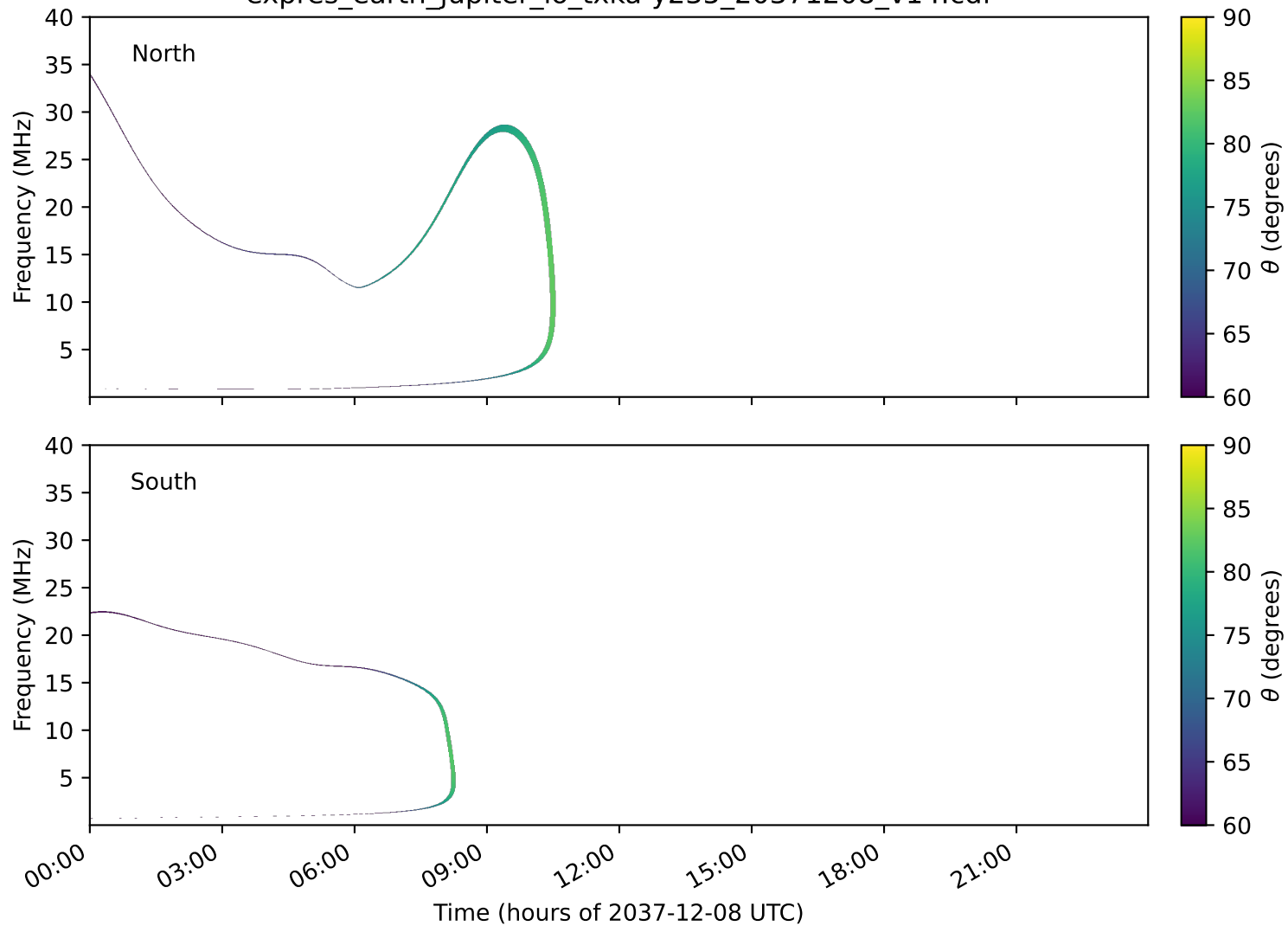
expres_earth_jupiter_io_txka-y235_20371208_v14.cdf
