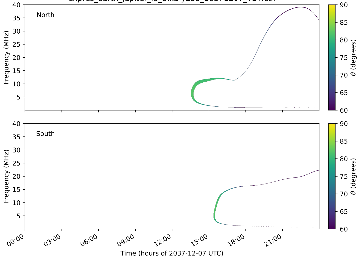
expres_earth_jupiter_io_txka-y235_20371207_v14.cdf
