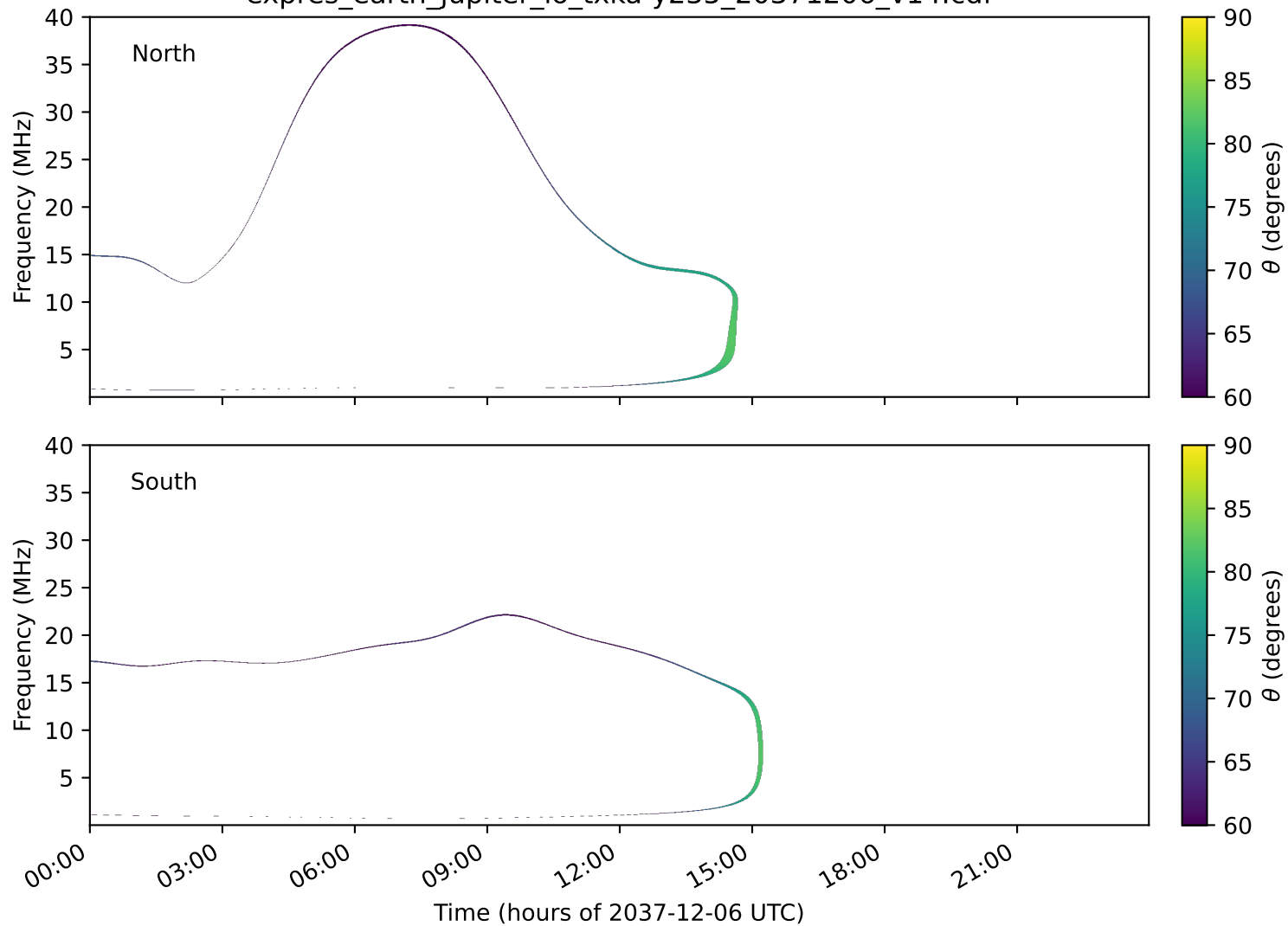
expres_earth_jupiter_io_txka-y235_20371206_v14.cdf
