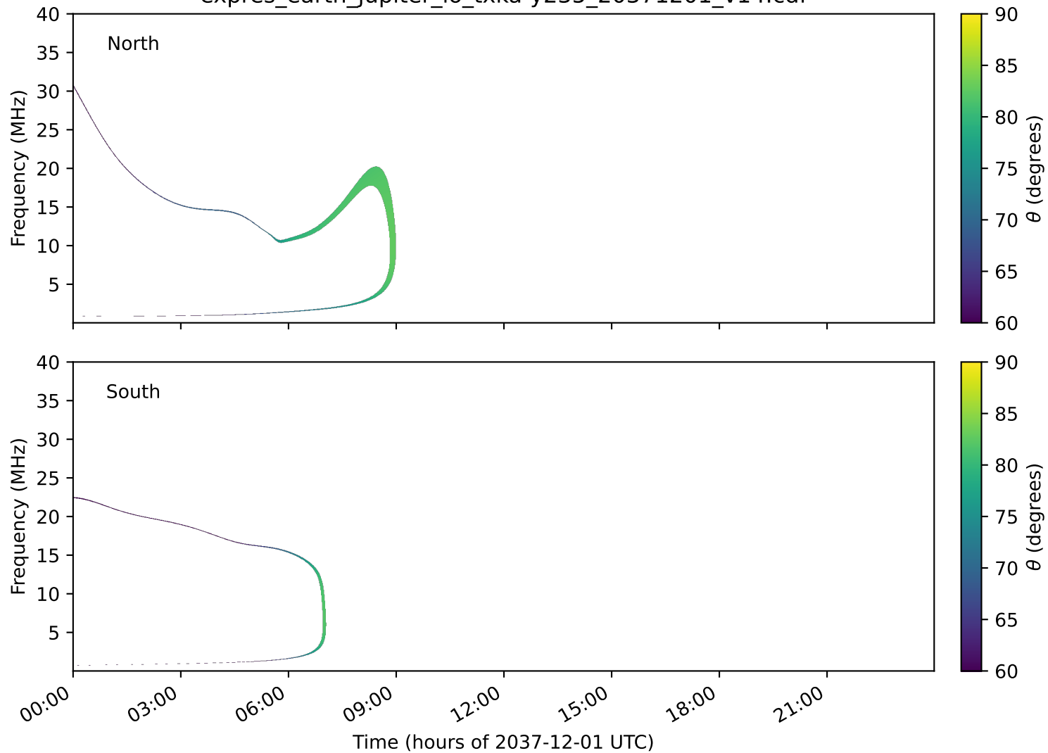
expres_earth_jupiter_io_txka-y235_20371201_v14.cdf
