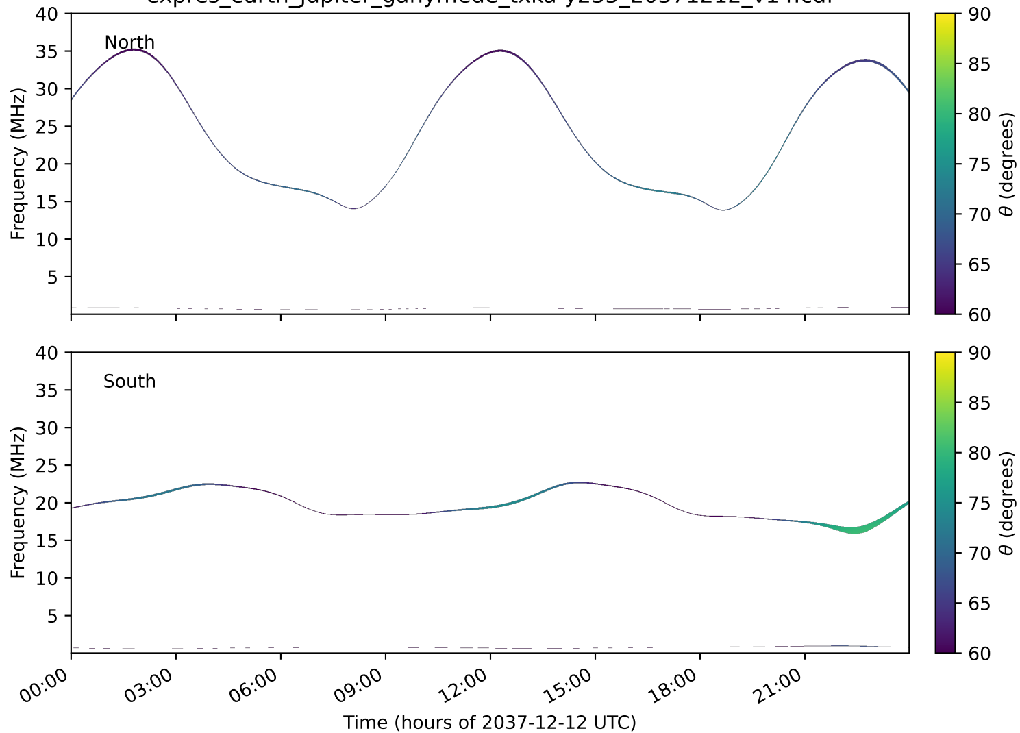
expres_earth_jupiter_ganymede_txka-y235_20371212_v14.cdf
