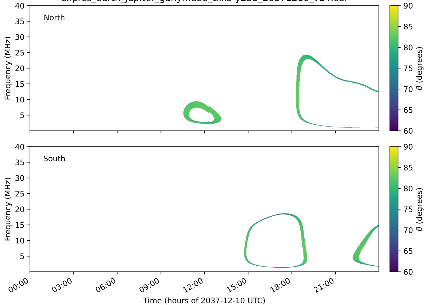
expres_earth_jupiter_ganymede_txka-y235_20371210_v14.cdf
