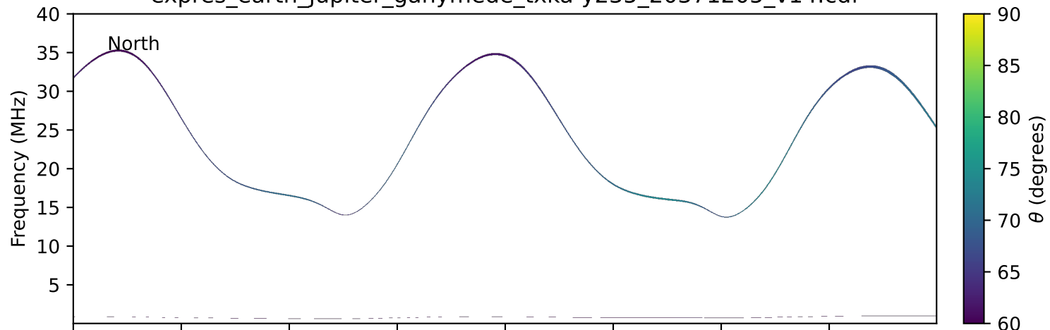
expres_earth_jupiter_ganymede_txka-y235_20371205_v14.cdf
