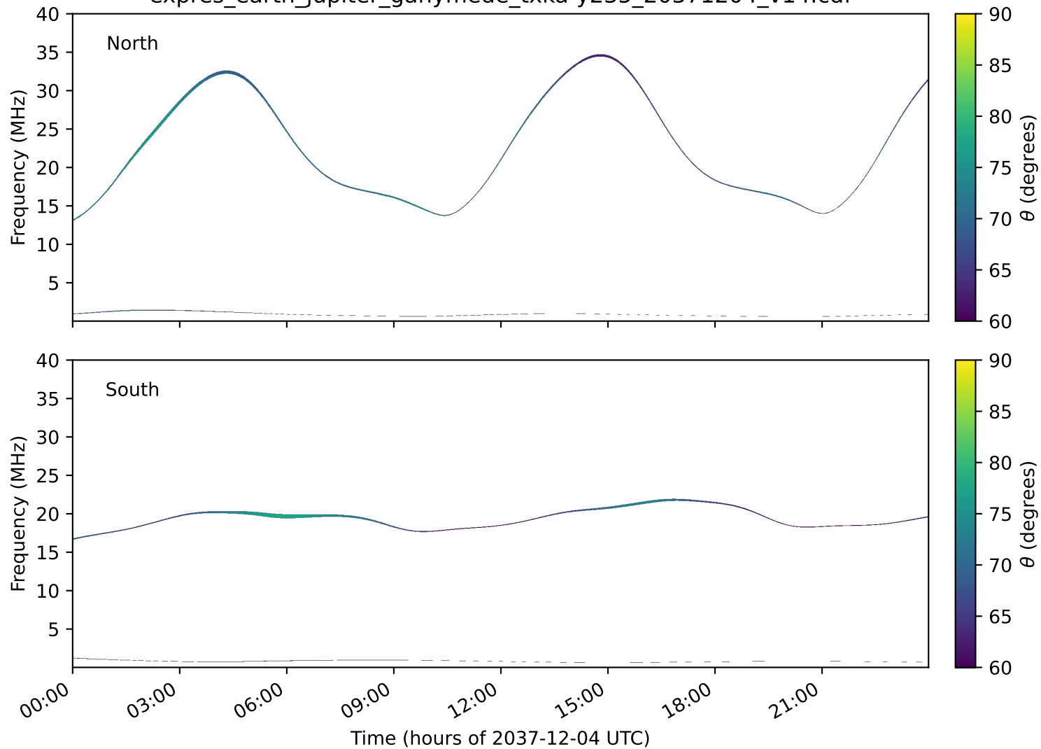
expres_earth_jupiter_ganymede_txka-y235_20371204_v14.cdf
