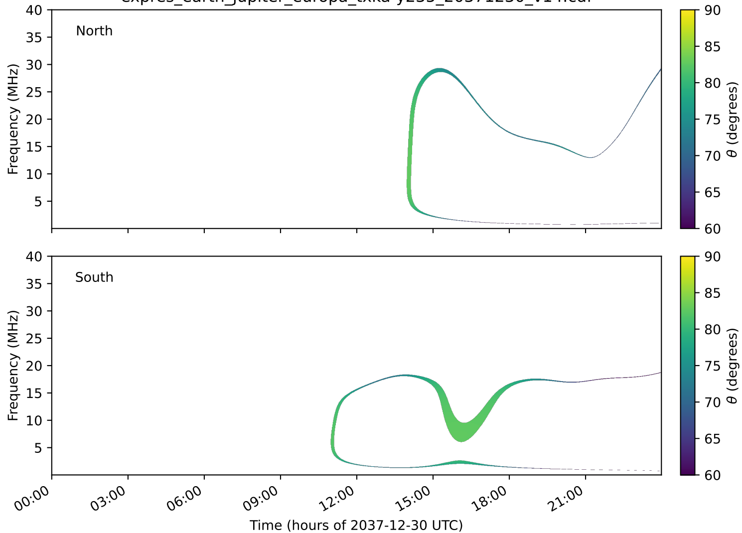
expres_earth_jupiter_europa_txka-y235_20371230_v14.cdf
