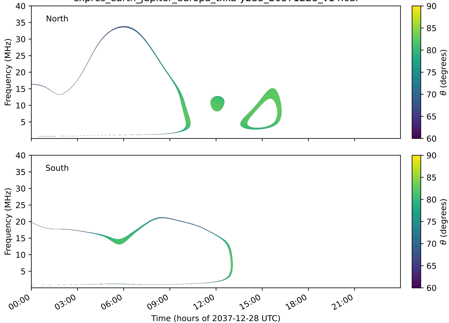
expres_earth_jupiter_europa_txka-y235_20371228_v14.cdf
