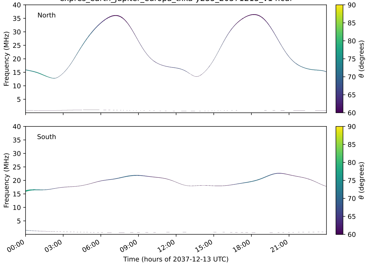
expres_earth_jupiter_europa_txka-y235_20371213_v14.cdf
