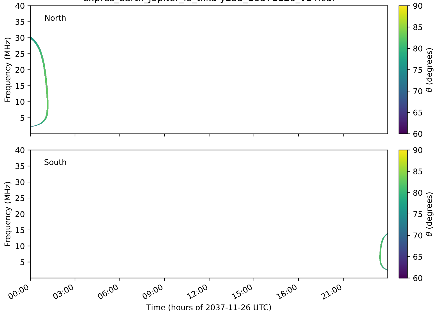
expres_earth_jupiter_io_txka-y235_20371126_v14.cdf
