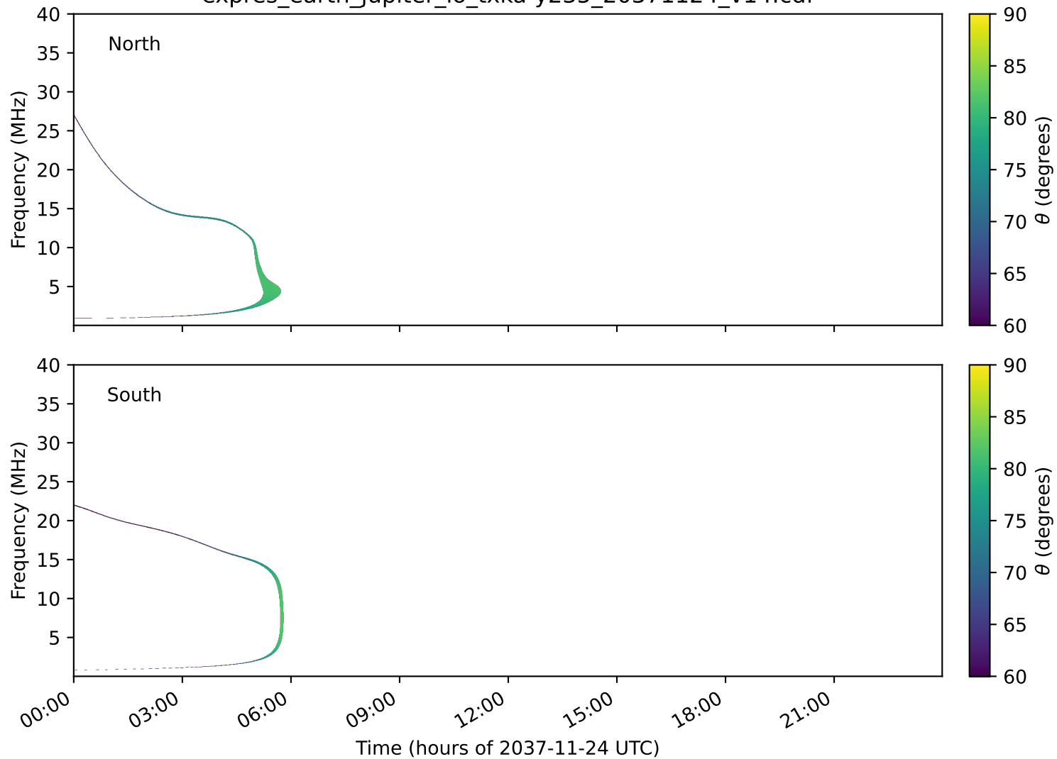
expres_earth_jupiter_io_txka-y235_20371124_v14.cdf
