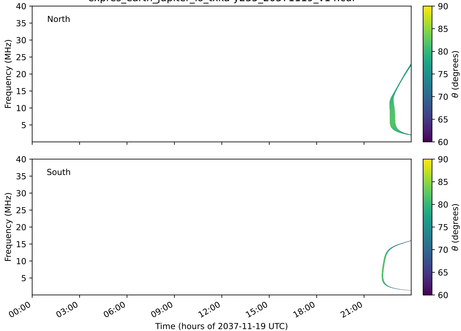
expres_earth_jupiter_io_txka-y235_20371119_v14.cdf
