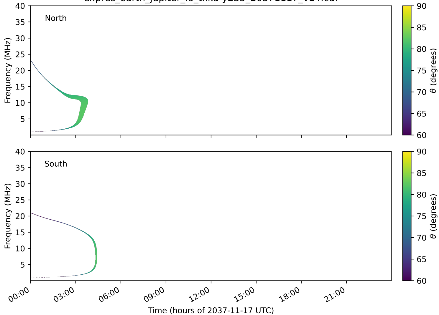
expres_earth_jupiter_io_txka-y235_20371117_v14.cdf
