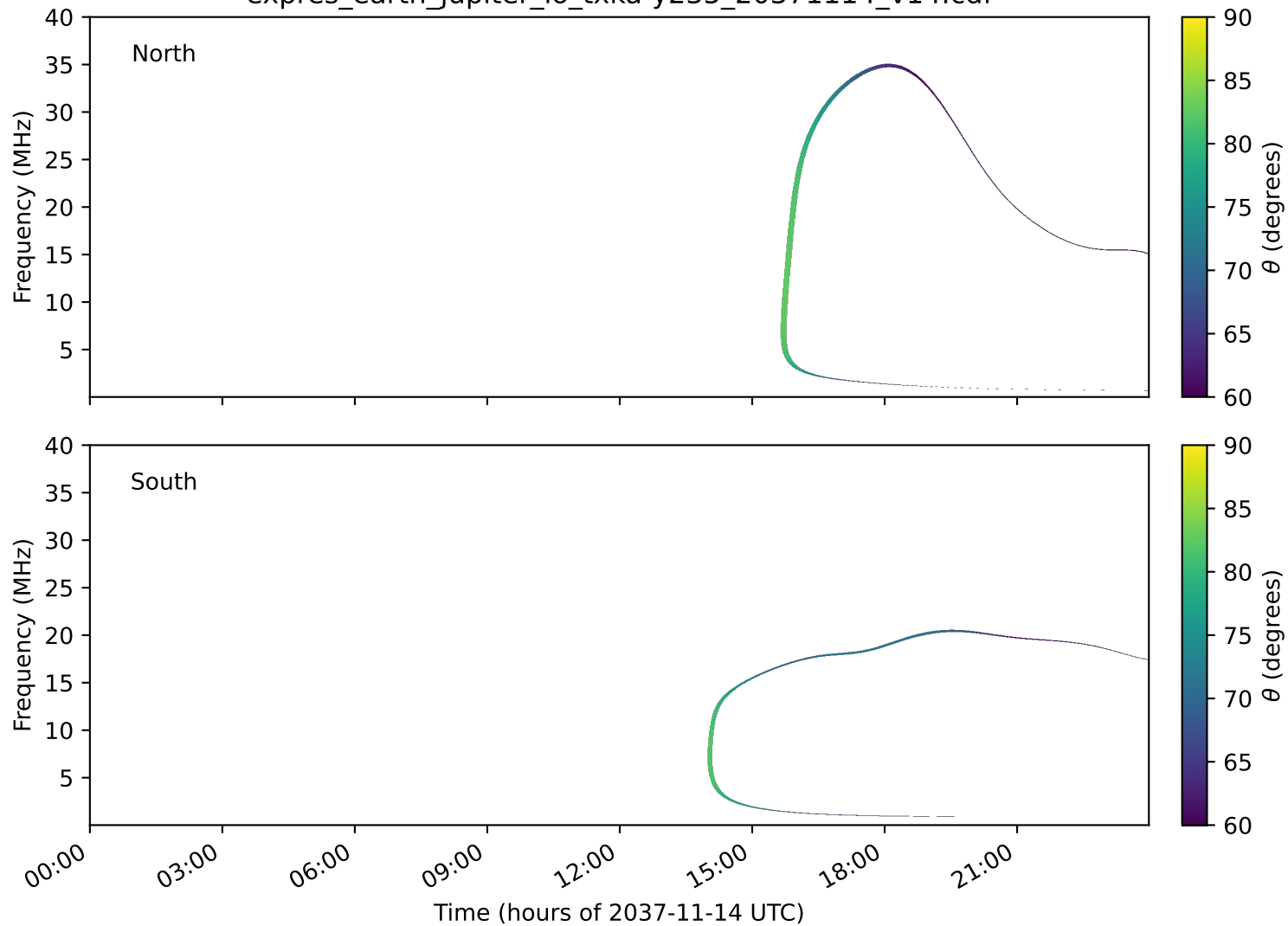
expres_earth_jupiter_io_txka-y235_20371114_v14.cdf
