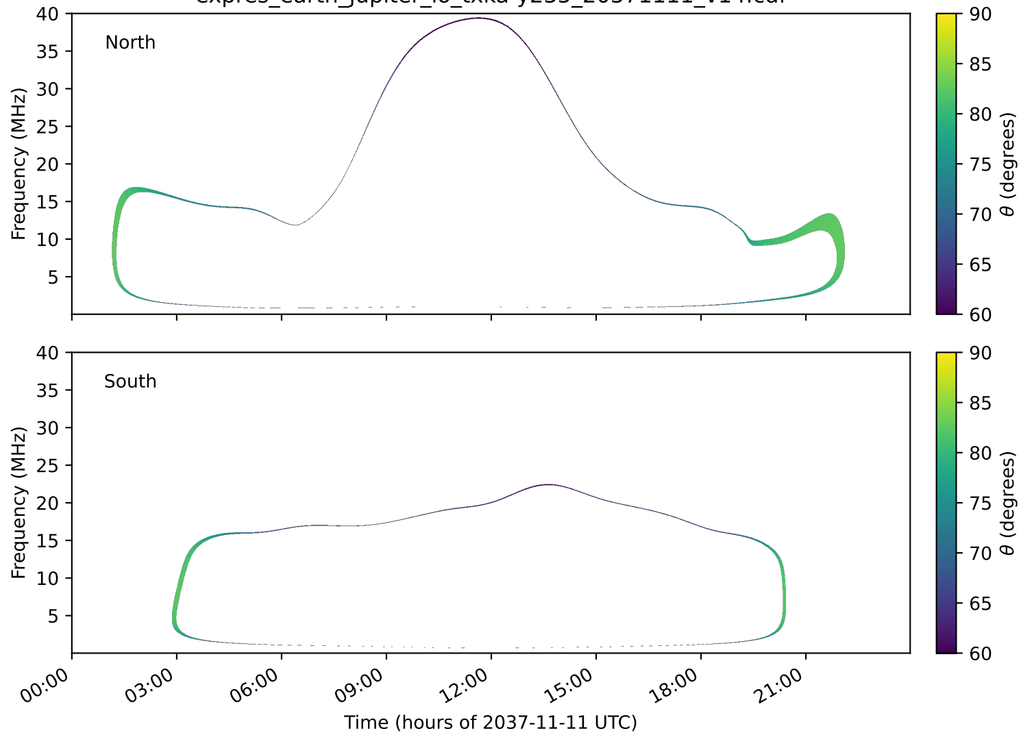
expres_earth_jupiter_io_txka-y235_20371111_v14.cdf
