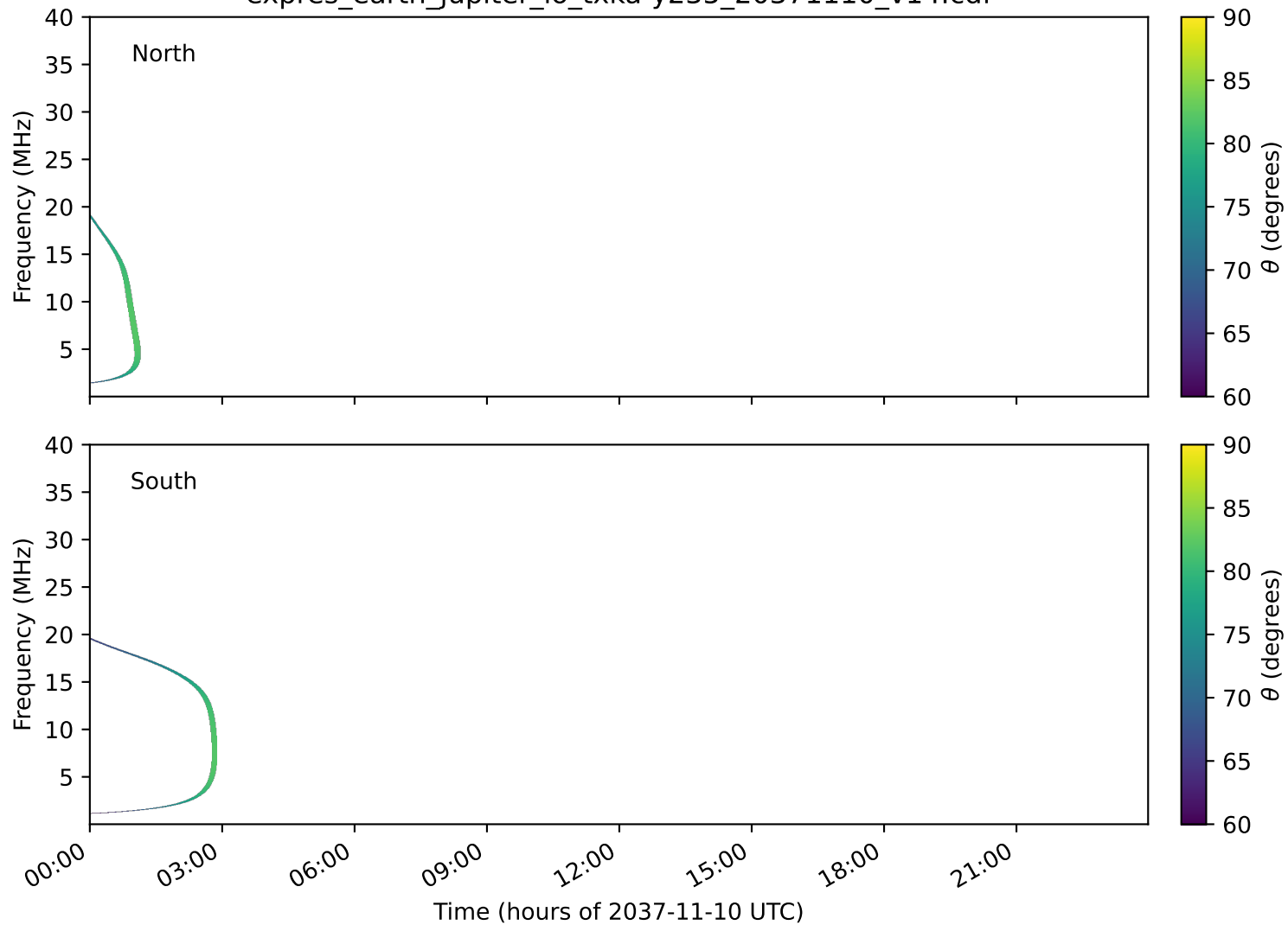
expres_earth_jupiter_io_txka-y235_20371110_v14.cdf
