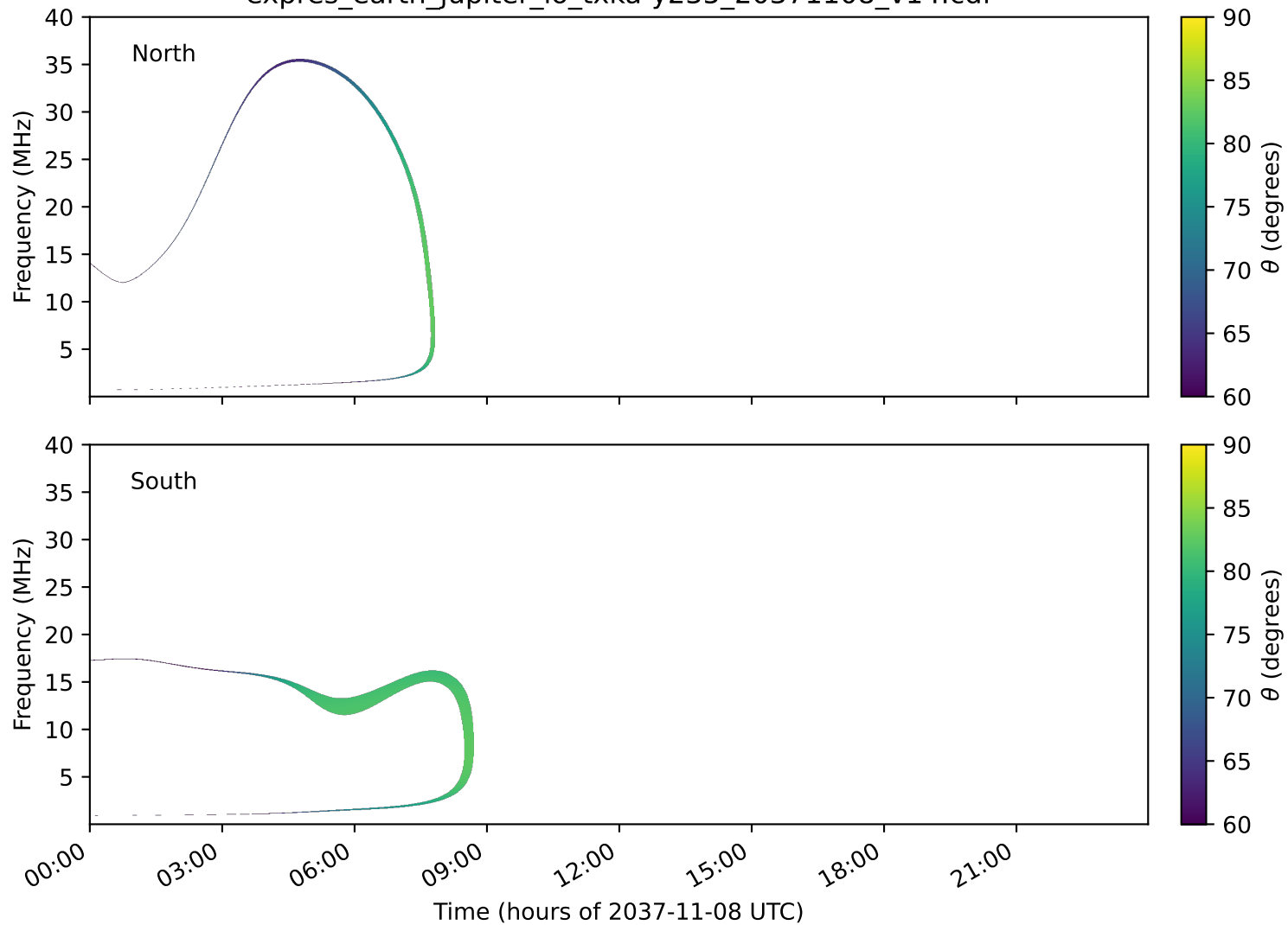
expres_earth_jupiter_io_txka-y235_20371108_v14.cdf
