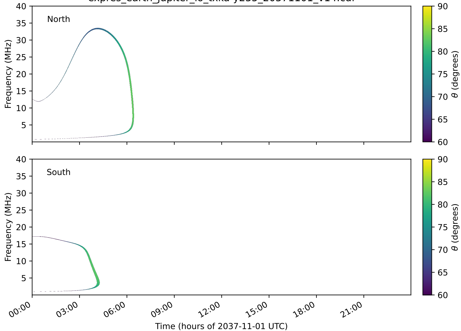
expres_earth_jupiter_io_txka-y235_20371101_v14.cdf
