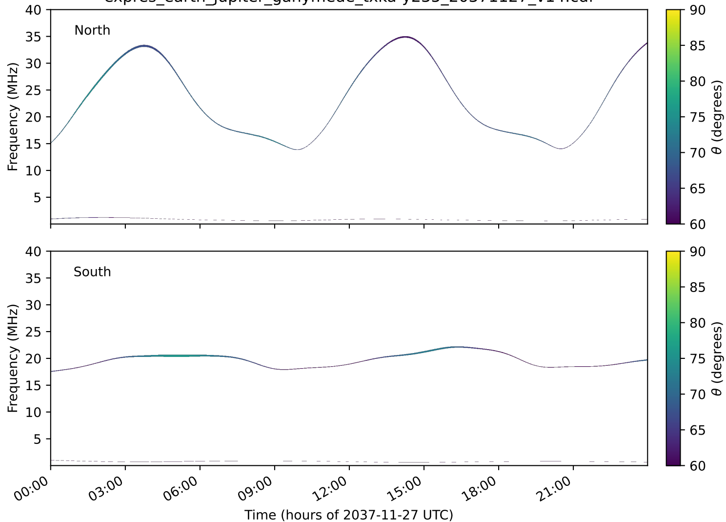
expres_earth_jupiter_ganymede_txka-y235_20371127_v14.cdf
