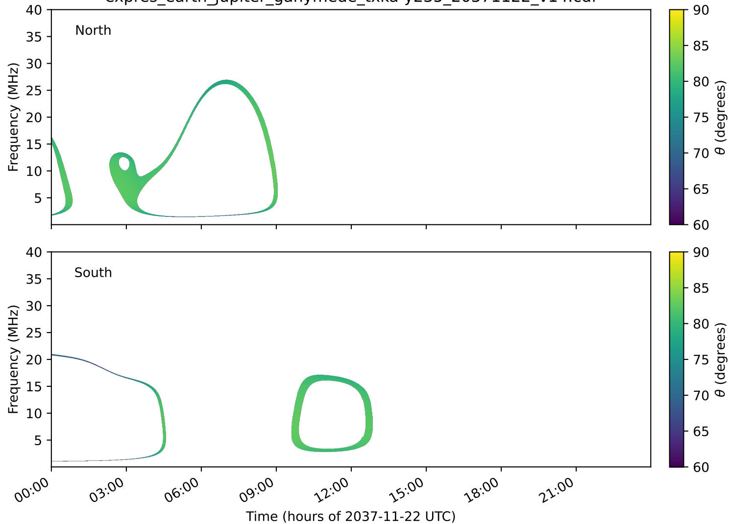
expres_earth_jupiter_ganymede_txka-y235_20371122_v14.cdf
