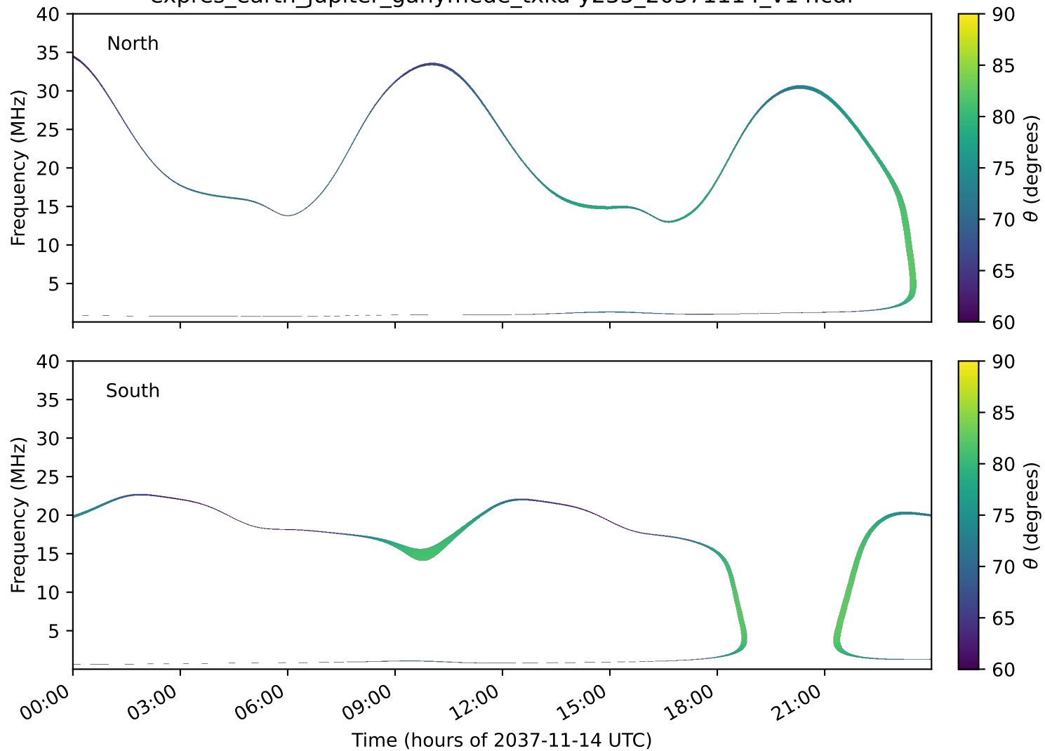
expres_earth_jupiter_ganymede_txka-y235_20371114_v14.cdf
