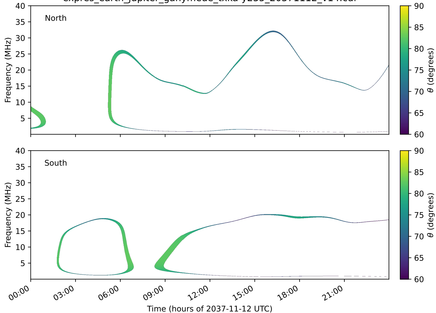
expres_earth_jupiter_ganymede_txka-y235_20371112_v14.cdf
